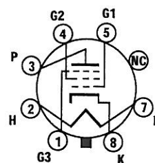
Octal Base Connections
