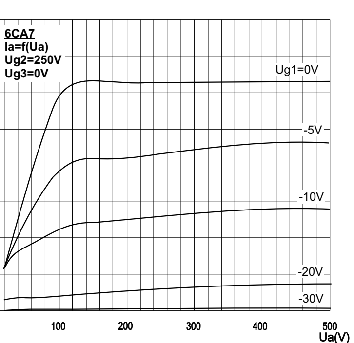
PLATE CHARACTERISTICS
