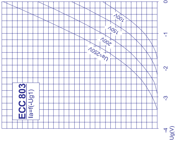
TRANSFER CHARACTERISTICS
