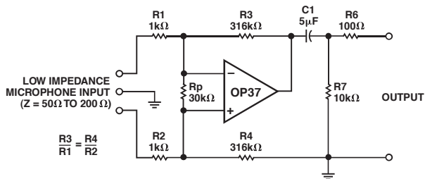
Figure 10. Fixed Gain Transformerless Microphone Preamp
