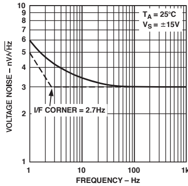
TPC 2. Voltage Noise Density vs. Frequency
