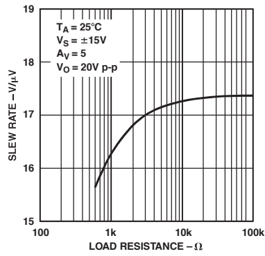
TPC 32. Slew Rate vs. Load
