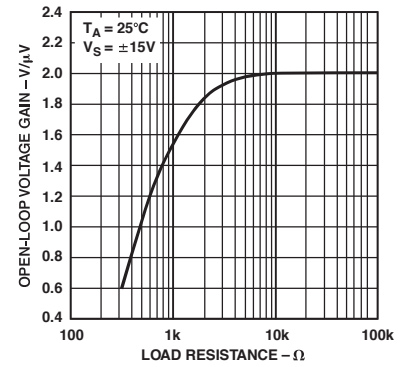
TPC 30. Open-Loop Voltage Gain vs. Load Resistance
