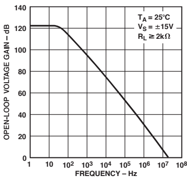
TPC 16. Open-Loop Gain vs. Frequency
