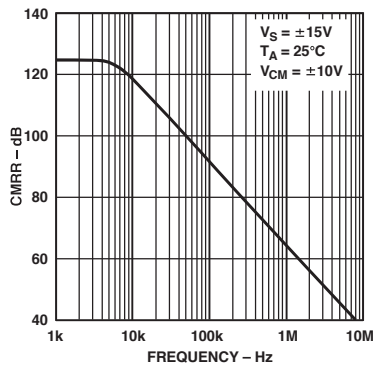
TPC 26. CMRR vs. Frequency
