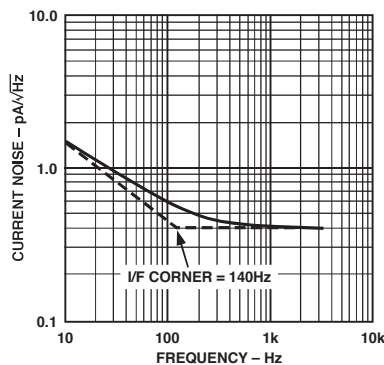
TPC 8. Current Noise Density vs. Frequency
