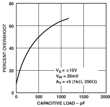
TPC 22. Small-Signal Overshoot vs. Capacitive Load
