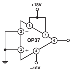
Figure 3. Burn-In Circuit
