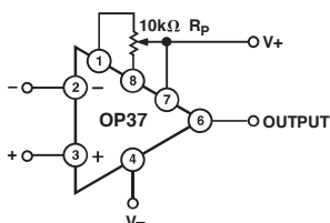
Figure 1. Offset Nulling Circuit
