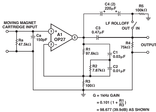
Figure 8. Phono Pre-Amplifier Circuit
