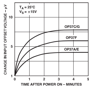
TPC 12. Warm Up Offset Voltage Drift
