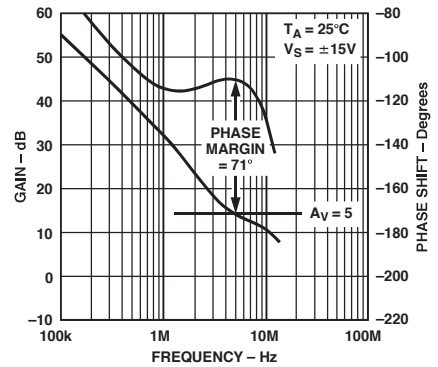
TPC 18. Gain, Phase Shift vs. Frequency
