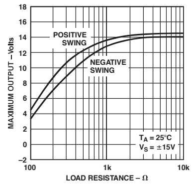
TPC 21. Maximum Output Voltage vs. Load Resistance
