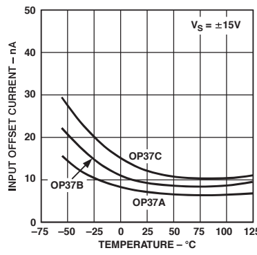
TPC 15. Input Offset Current vs. Temperature
