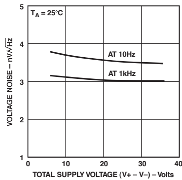
TPC 7. Voltage Noise Density vs. Supply Voltage
