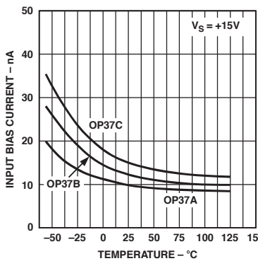
TPC 14. Input Bias Current vs. Temperature
