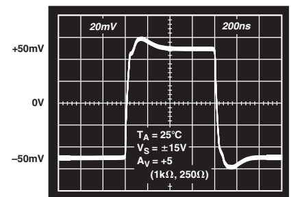
TPC 24. Small-Signal Transient Response
