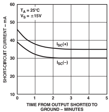
TPC 25. Short-Circuit Current vs. Time
