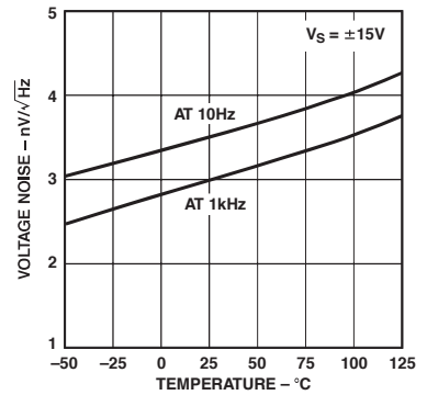
TPC 6. Voltage Noise Density vs. Temperature
