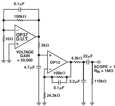
TPC 28. Noise Test Circuit (0.1 Hz to 10 Hz)
