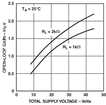
TPC 19. Open-Loop Voltage Gain vs. Supply Voltage
