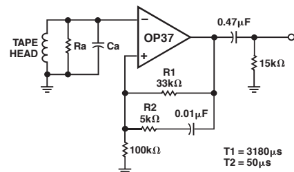
Figure 9. Tape-Head Preamplifier
