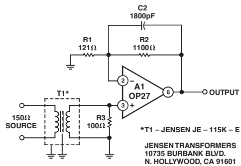
Figure 11. Microphone Transformer Coupled Preamp
