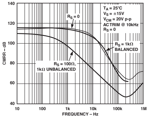
Figure 4b. CMRR vs. Frequency
