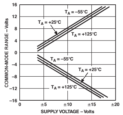
TPC 27. Common-Mode Input Range vs. Supply Voltage
