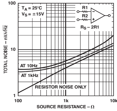
TPC 5. Total Noise vs. Source Resistance
