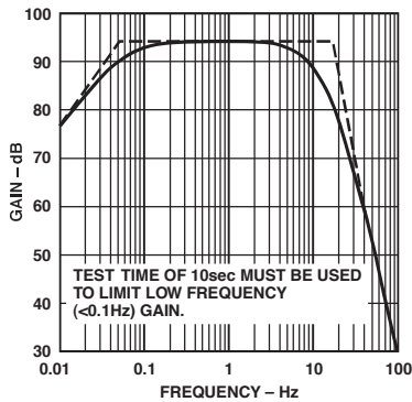
TPC 1. Noise-Tester Frequency Response (0.1 Hz to 10 Hz)
