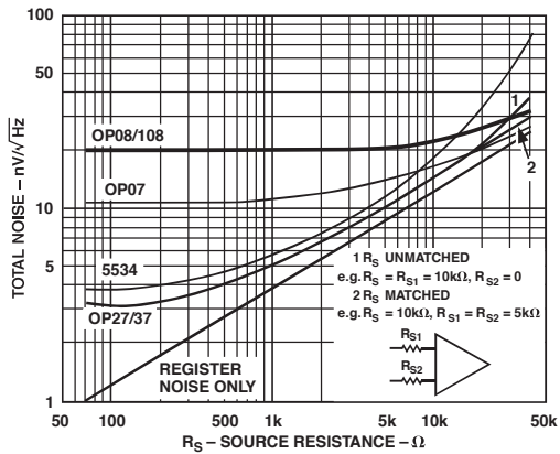
Figure 5. Noise vs. Resistance (Including Resistor Noise @ 1000 Hz)
